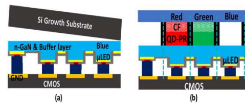
Fig 2. Schematic of (a) the blue GaN micro-LED array integrated with the CMOS backplane, and (b) the full-color micro-display with QDs-based color conversion layer
