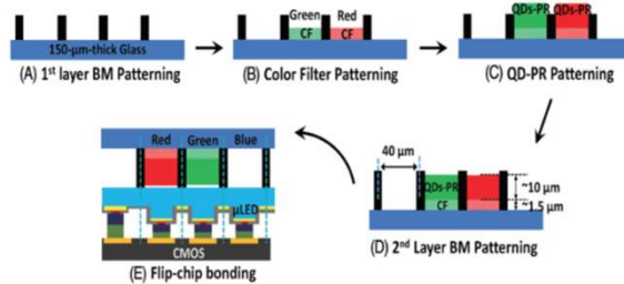
Fig 1. Process flow of the color conversion layer using quantum dots photoresist (QDs-PR)
